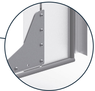
MAGNELIS® REINFORCEMENT CORNER BRACKETS
